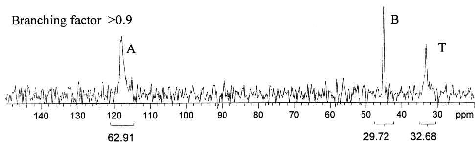
Fig. 16. Quantitative 15 N NMR spectrum (D 2 O); polymer prepared from N -acryloyl-1,2-diaminoethane hydrochloride (pH 1).
